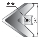
SALFORD Láb (260 mm) P33.260604.00 W=1,91 kg
