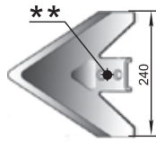
SALFORD Láb (240 mm) P33.240604.00 W=1,84 kg
