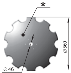
Korong БДМ P33.1905-22 M=10,97 kg
