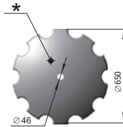
Korong БДТ P33.428.001 lap-10 (boronára) M=15,5 kg
