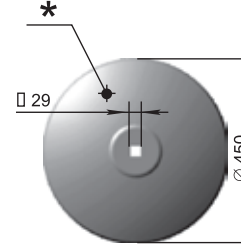
Korong ЛДГ C-1-1-450-5-29 P33 407.001 M=6,3 kg
