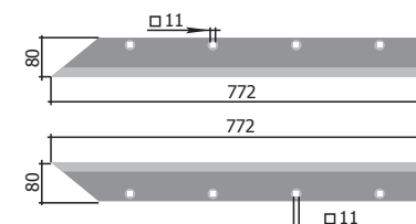
Brăzdar stâng P33 KWA 07.030, drept P33 KWA 07.030-01 M (uneia)=3,53 kg
