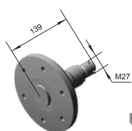
Butuc P33.18.14.103 M=4,43 kg
